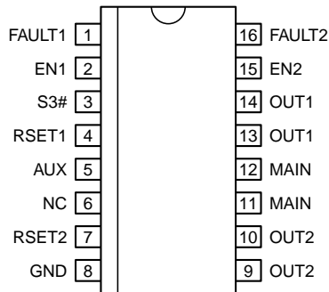
16-Pin QSOP (QS)
